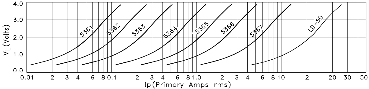
The output of the 5360 series of load detectors when terminated with a 100 ohm resistor. Ip ranging from 0.25 to 2.5 times the rated current.
