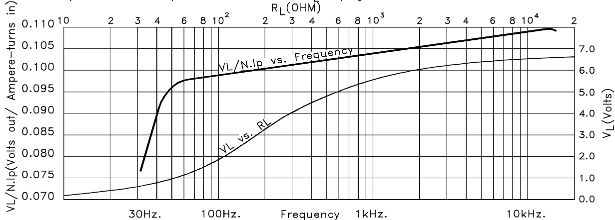
VL/N.Ip vs. Frequency curve shows the output of the load sensor as a function of frequency across a 100 ohm terminating resistor at rated primary current. (20A for LD-50)
